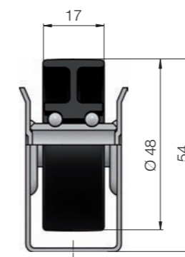
Fig.: Dimensions with polymer conveyor wheels
