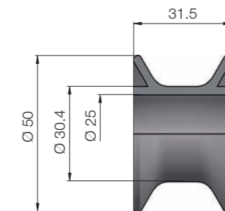
Fig.: Dimensions for K 212
