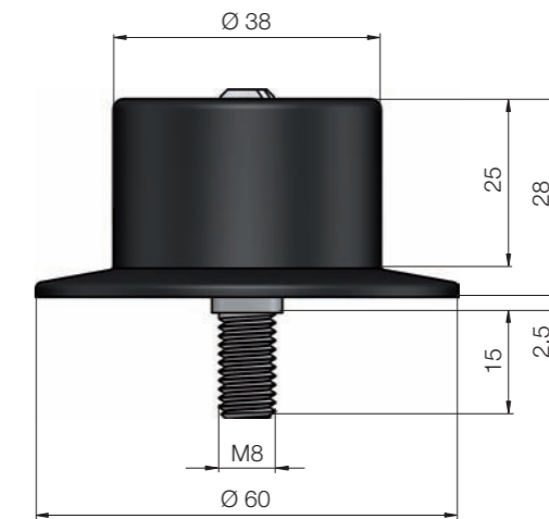
Fig.: Dimensions with flange
