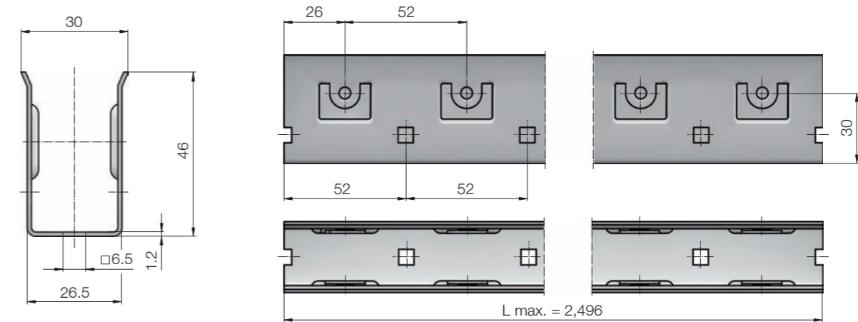
Fig.: Dimensions of steel profile Fig.: Dimensions of Roller Track
